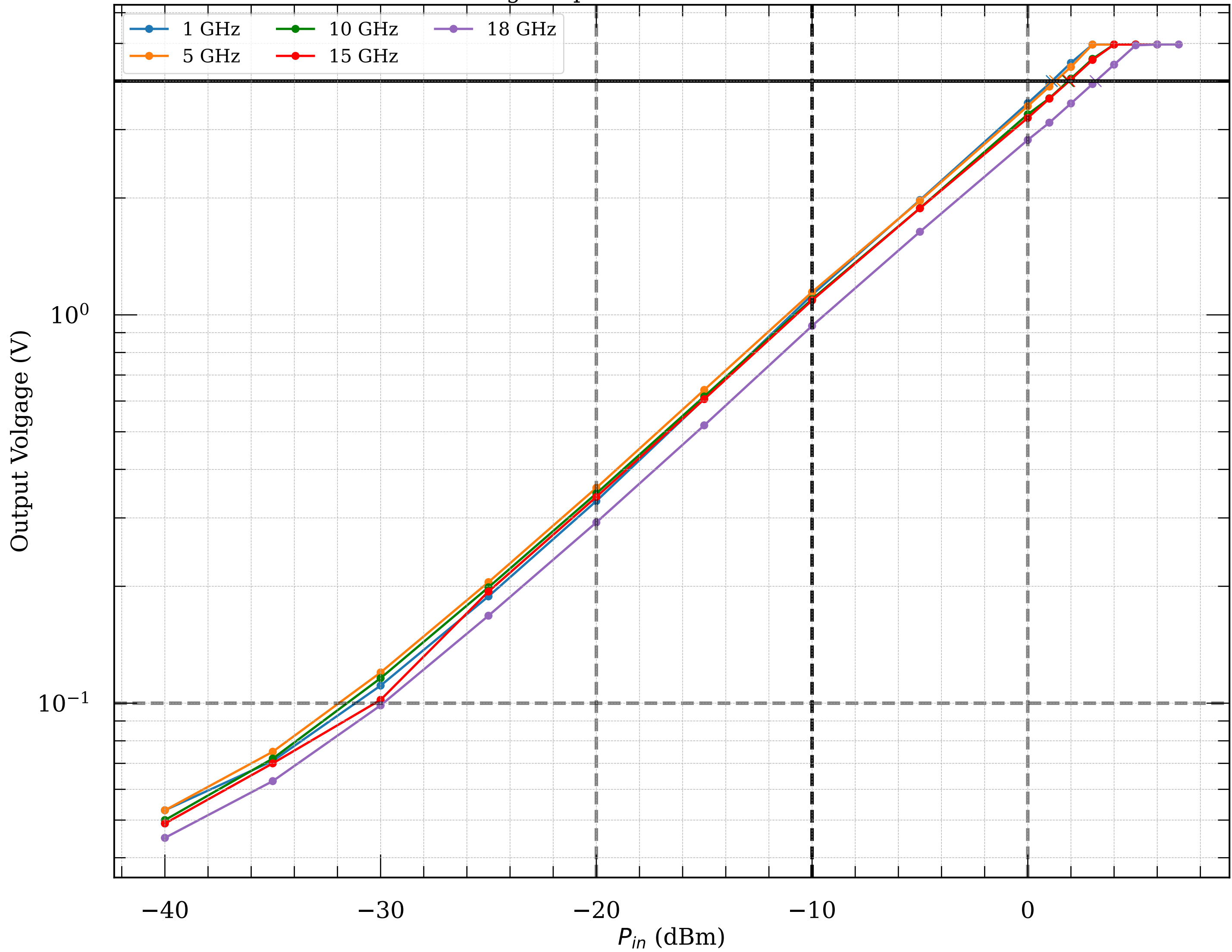
Measured voltage-to-power curve of detector module018v2
